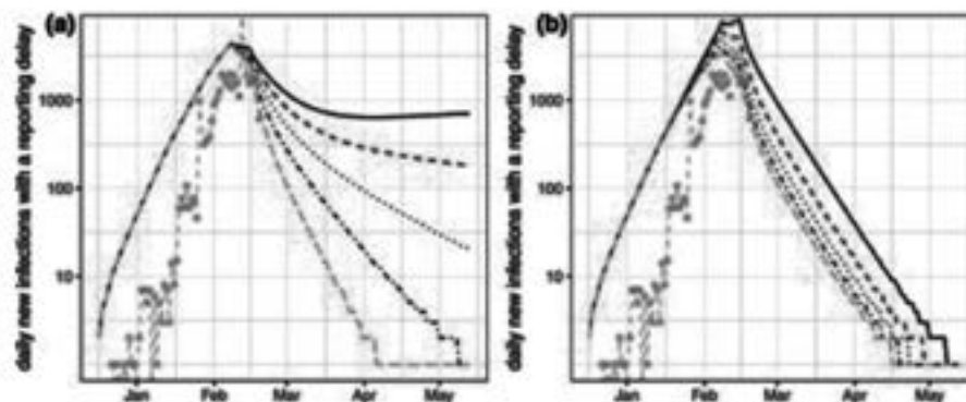
Figure 5 Sensitivity analyses on a and \kappa . We simulate the base model with both individual reaction and governmental action while varying a and \kappa . We show model outcome when (a) a = 0.5 (black solid), 0.6 (red dashed), 0.7 (green dotted), 0.8 (blue dash-dotted) and 0.9 (cyan long dashed curve), while \kappa = 1117.3 , when (b) \kappa = 100 (black solid), 500 (red dashed), 900 (green dotted), 1300 (blue dash-dotted) and 1700 (cyan long dashed curve), while a = 0.8478 . Grey dots show the reported cases.
